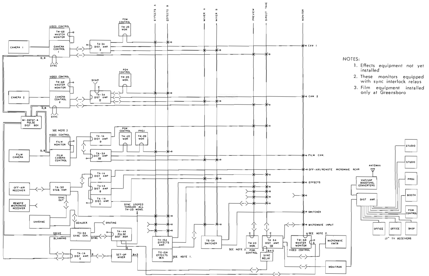
FIG. 54. Common video system used at all WUNC-TV studios.
