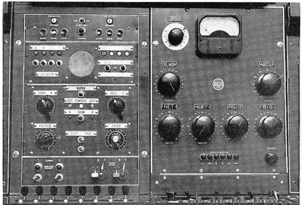
FIG. 21. KOMO-TV master control console. On the left Section 1 contains a TK-21A vidicon film camera control, Section 2 a TK-20D iconoscope slide camera chain; Sections 3 and 4 are projector remote controls and an RCA TC-4 audio/video switcher (shown in more detail in Figure 22). Section 5 contains a TS-10 switcher and line out master monitor; Section 6 a preview monitor, the input controlled by a 12-position, push-button switch located on the sloping section of the console desk. The last section contains stab, amp controls and projector controls for the RCA TP-16 and TP-3 projectors used on the 3-V System.
