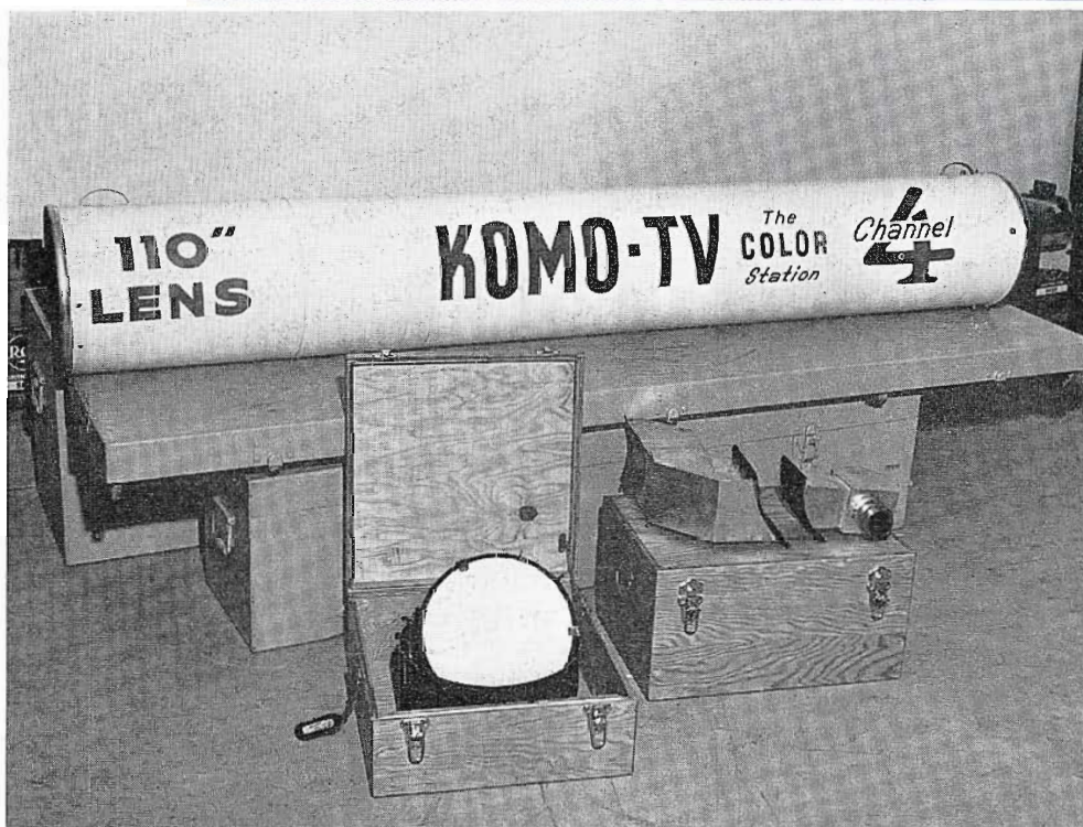
FIG. 30. Designed and built by Howard Moses, of the KOMO-TV Engineering Staff, the 110-inch lens is constructed of a 12-inch diameter Fiberglas tube, 7 feet long. At the rear end is mounted an aluminized front surface parabolic mirror. This was ground from a 2-inch Pyrex blank, 10 inches in diameter. It brings light rays to a focus at a point 110 inches from its surface. In the forward part of the tube is a diagonal mirror. It reflects the light rays through a series of front surface mirrors, contained in a light-tight housing between lens and TV camera, to one port in the turret. The image is formed at the photo-cathode of the image orthicon camera tube. Lens and mirror construction are highly accurate, there is minimum light loss and color aberration. An 80-inch lens can also be accommodated in the same tube in place of the 110-inch lens. A smaller tube is used to accommodate a 50-inch lens. The tube is held in place by a Duralumin framework that fastens to the TV camera. The tubes are painted white to prevent thermal air currents from rising inside, which would cause optical aberrations. Each tube is complete in its own special packing case as shown. The mirrors and light chambers are carried in separate cases. These lenses are used with black-and-white cameras only.
