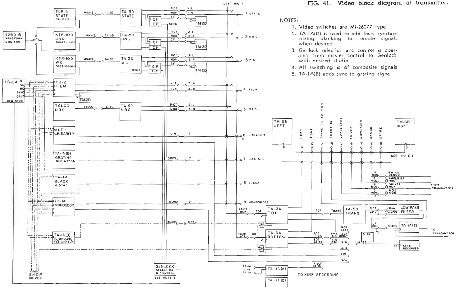
FIG. 41. Video block diagram at transmitter.
