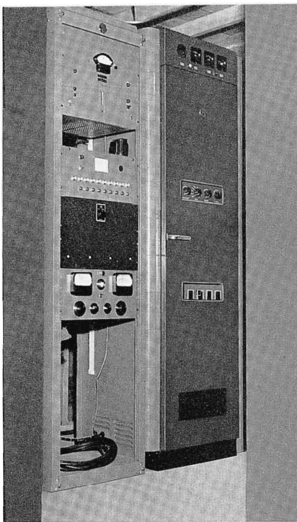
FIG. 17. The KBZY transmitter building houses rack of remote-control equipment and BTA-250M Transmitter.
