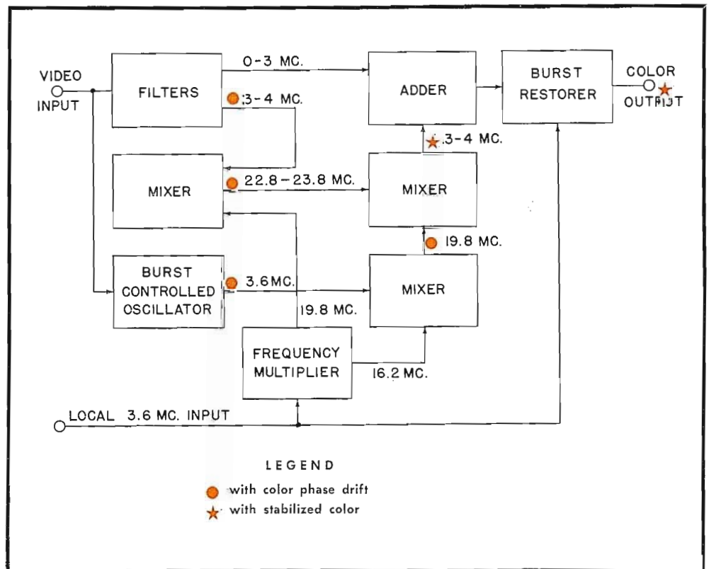
FIG. 2. Simplified block diagram of color processing circuits.
