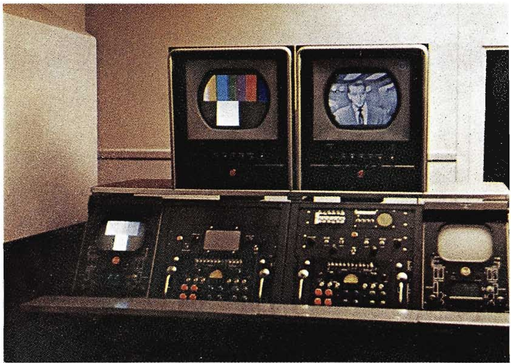
FIG. 36. TK-41 color camera control room console consisting of monitors and control equipment for two live color cameras. This room also contains an equipment rack housing the two colorplexers associated with the cameras. Windows opening out into Studio B at the right.
