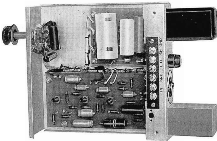
FIG. 5. This is the BA-26A with the cover removed. The preamplifier and its power supply are built on separate etched wiring circuit boards. The response selector switch (left) is mounted at the top of the chassis. This type of construction provides trouble-free operation.
