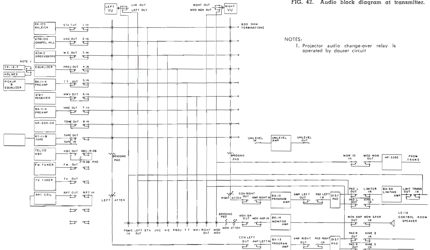
FIG. 42. Audio block diagram at transmitter.
