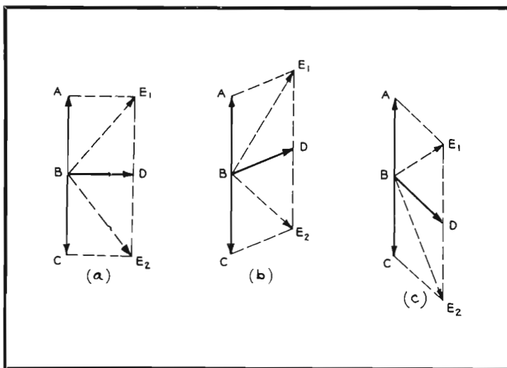
FIG. 3. Vector representation of frequency detector signal voltages.
