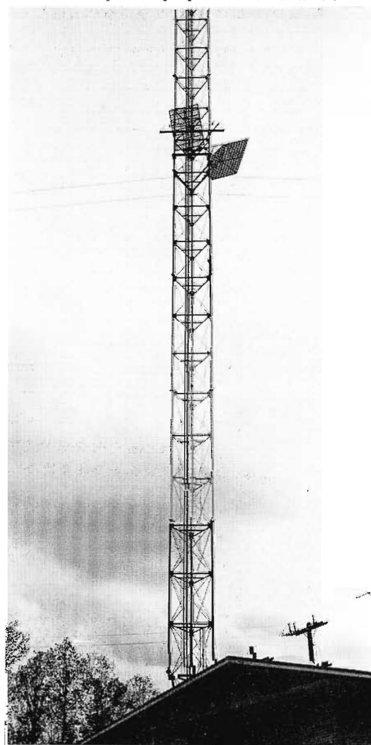
FIG. 37. Note passive microwave reflectors mounted part way up the antenna tower.
