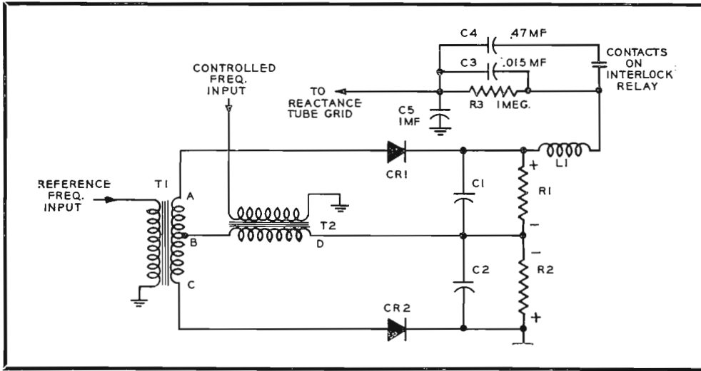
FIG. 2. Schematic diagram of the detector circuit.
